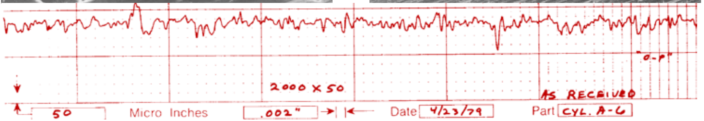
AS RECEIVED, PRODUCTION RIGID HONED, "O" photo at 1000X, "P" at 100X. Undirectional cut pattern from rigid hone operation. Peaky profile with typical saw tooth appearance. 20 to 25 \mu " finish. #A-6 cylinder.
