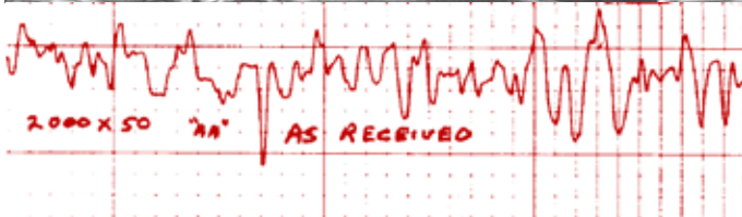
AS RECEIVED RIGID HONED BY FACTORY REWORK SECTION. "AA" photo at 1000X. Uniform cross-hatch pattern. Smeared, torn, and folded metal, smeared metal loosely attached. Very peaky profile.. 25 to 35 \mu " (.63 to .89 \mu m) finish. Cylinder #B-2.
