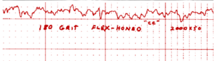
AFTER FLEX-HONE, 180 grit silicon carbide "CC" photo at 1000X. Uniform cross-hatch pattern. Surface has clean open appearance with most of torn, folded, and smeared metal removed. Excellent semi - plateaued profile. 20 to 25 \mu " (.51 to .63 \mu m) finish. Cylinder #B-2.
