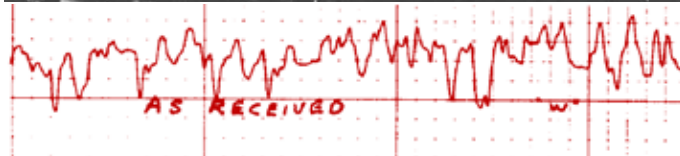
AS RECEIVED RIGID HONED BY FACTORY REWORK SECTION. "W" photo at 1000X. Cross-hatch has majority of cut in one direction. Smeared, torn, jagged and folded metal on surface. Smeared metal loosely attached to surface. Very peaky profile finish. 40 to 50 \mu " (1.02-1.27 \mu m) finish. Cylinder #B-1.
